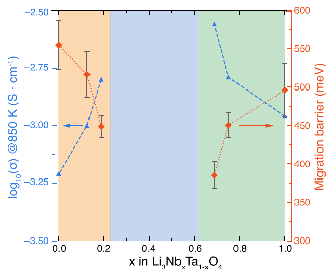
Figure 4. Temperature-dependent ionic conductivities \sigma (in \text{S}\cdot\text{cm}^{-1} ) (at 850 K) and Arrhenius-fitted migration barriers (in meV) of Li 3 Nb x Ta 1-x O 4 for x = 0, 0.125, 0.1875, 0.6875, 0.75, \text{ and } 1 derived from machine learning MTP molecular dynamics calculations. Colored regions represent the phase distributions at 300 K: \alpha phase, x = 0.00\text{--}0.23 , \alpha + \beta phases, x = 0.23\text{--}0.62 , \beta phase, x = 0.62\text{--}1.00 . The error bars of migration barriers fitted from the temperature-dependent Li + diffusivities are shown.
