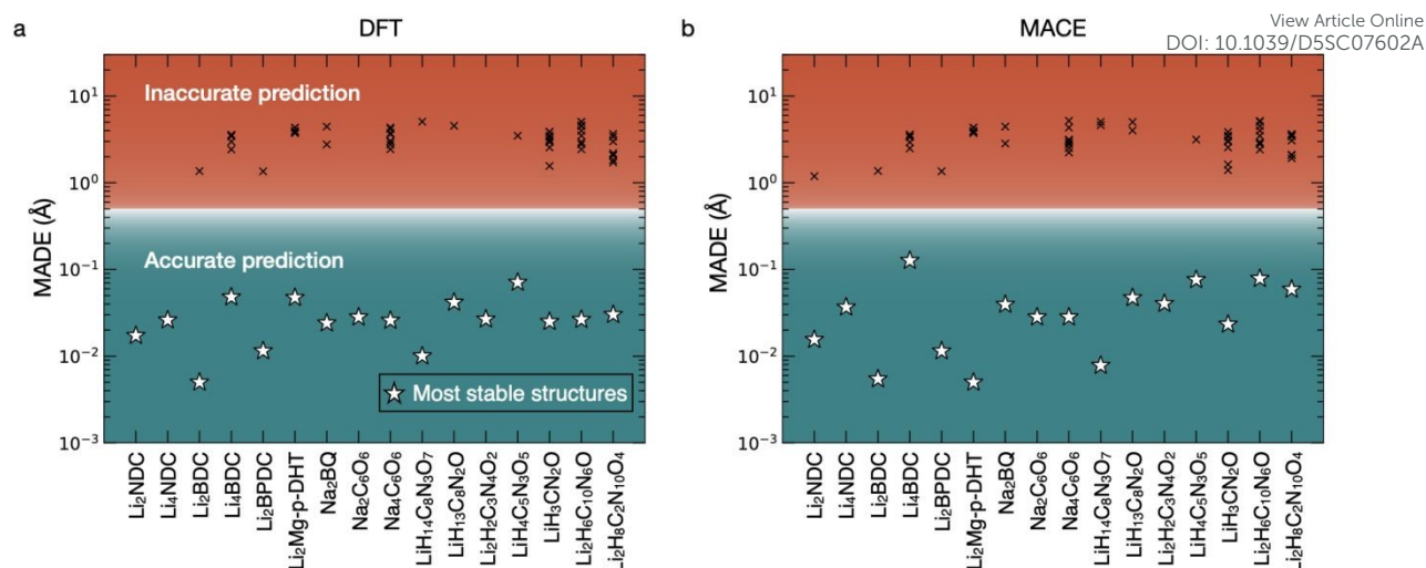
Figure 4: Accuracy of the predicted active ion positions with the proposed SIIE workflow and ELIISE. MADE (Eq. 3) values determined after optimization of ionic positions with (a) first-principles DFT and (b) the machine learned potential MACE. Stars indicate the most stable (lowest total energy) ion arrangements in each organic structure, and crosses indicate the thermodynamically unfavorable (high energy) structures. Details of reference structures reported in the literature are in Table S1 .
