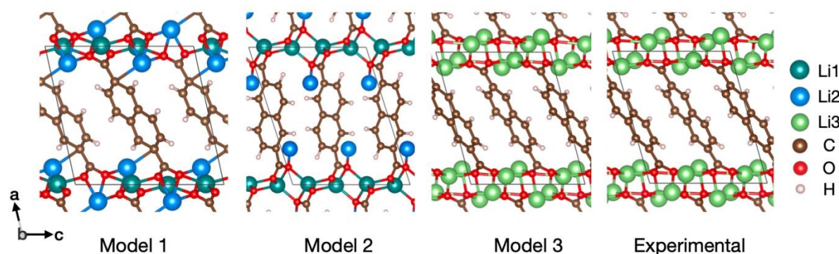
Figure 3: Li 4 NDC structures: Model 1, Model 2, Model 3, and experimentally refined from single-crystal XRD. 35 Different crystallographic Li sites are shown.
