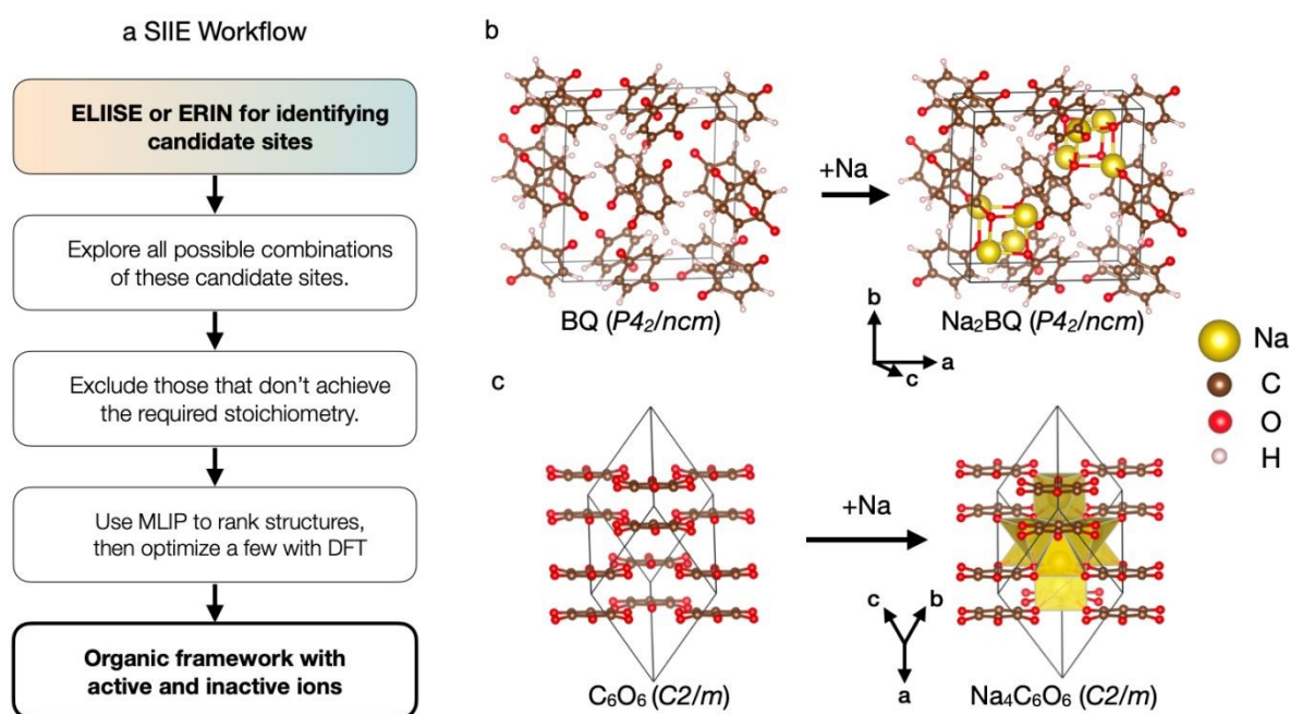
Figure 2: Workflow for the Simultaneous Ion Insertion and Evaluation (SIIE) method (a) and its application in two OEMs (b) Disodium 1,4-benzoquinone ( Na_2BQ ) and (c) Tetrasodium rhodizonate ( Na_4C_6O_6 ). Combining SIIE with ELIISE, the Na-ion positions are located in two exemplary OEMs 38,62
