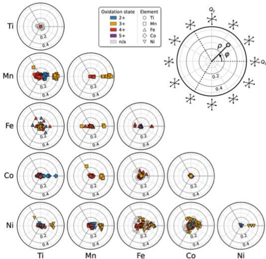
Figure 5. Q_2 – Q_3 Van Vleck distortion modes of the \text{TMO}_6 octahedra in the stable structures of all fifteen systems, arranged as in Figure 2 . Each point is one octahedron, with radius \rho (Å) giving the distortion magnitude and angle \phi its type. The schematic (top right) shows the O–TM–O axes every 30^\circ of \phi (outward arrows: elongation; inward: compression; dots: unchanged); dotted lines ( \phi = 0^\circ, 120^\circ, 240^\circ ) mark elongation along each axis. Colors denote oxidation state and markers the element; gray (n/a) marks structures where oxidation states violate charge neutrality.
