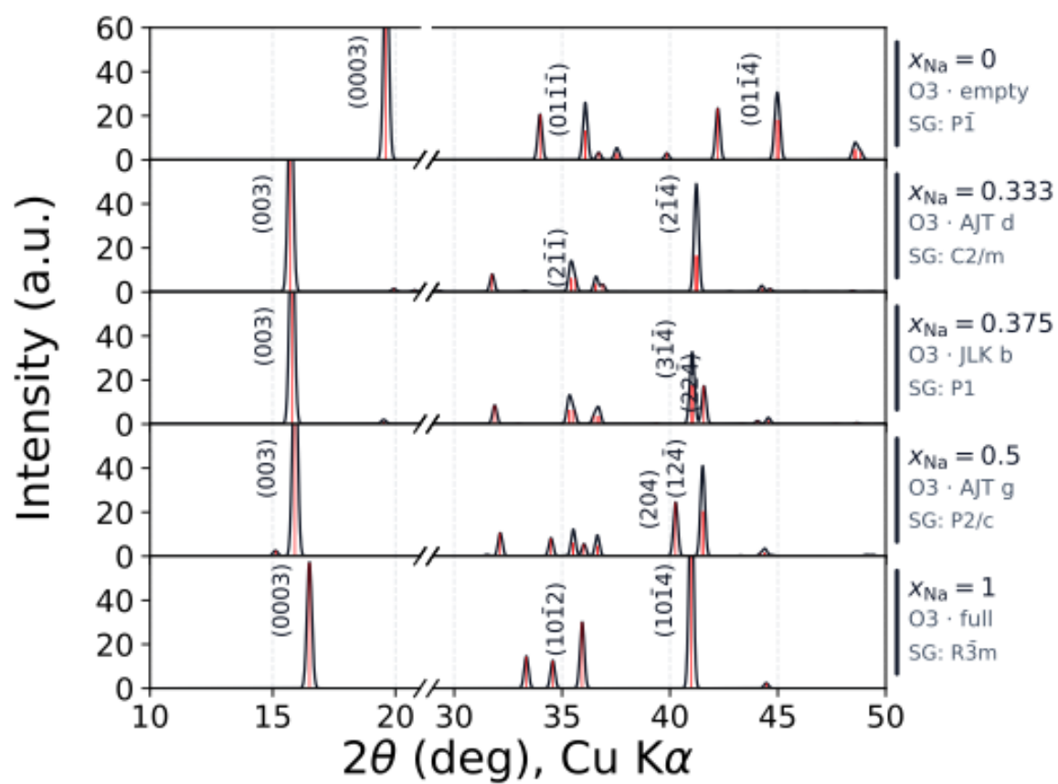
Figure S6 (continued). (c) \text{Na}_x\text{FeO}_2 .
