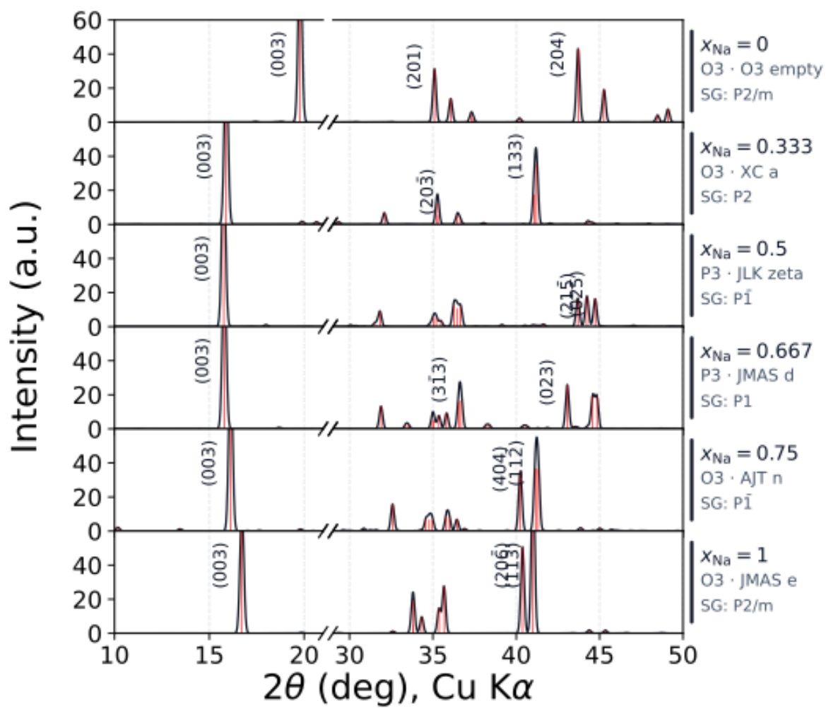
Figure S7 (continued). (b) \text{Na}_x\text{Ti}_{0.5}\text{Fe}_{0.5}\text{O}_2 .
