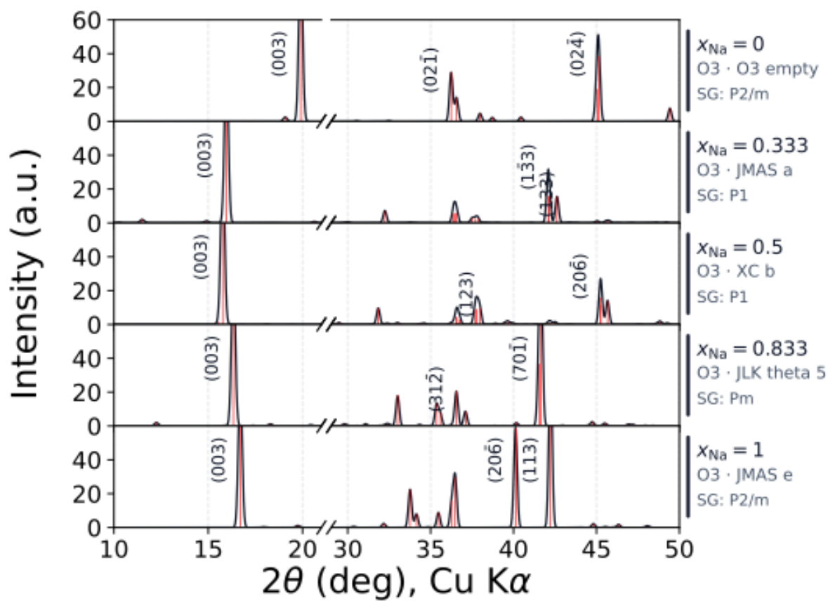
Figure S7 (continued). (c) \text{Na}_x\text{Ti}_{0.5}\text{Co}_{0.5}\text{O}_2 .
