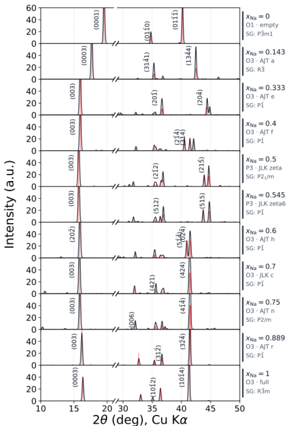
Figure S6. Simulated XRD patterns (Cu K \alpha ) of every hull-stable structure of the single-TM systems of Figure S3, one system per page, rows ordered by Na content. Black curves: Gaussian-broadened profiles ( \sigma = 0.10^\circ , FWHM \approx 0.24^\circ ); red sticks: underlying Bragg intensities; the three strongest reflections are labeled by their (hkl) indices; the 2\theta axis is broken between 21^\circ and 29^\circ . Right-hand labels give the Na content x_{\text{Na}} , the stable stacking and Na-vacancy ordering labels, and the space group of the relaxed structure. (a) \text{Na}_x\text{TiO}_2 .
