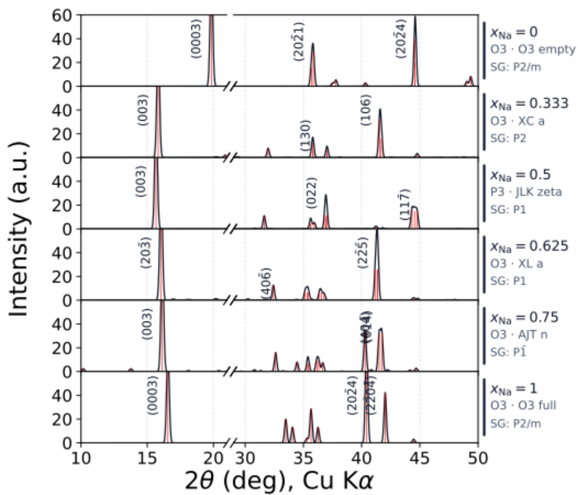
Figure S7 (continued). (e) \text{Na}_x\text{Mn}_{0.5}\text{Fe}_{0.5}\text{O}_2 .
