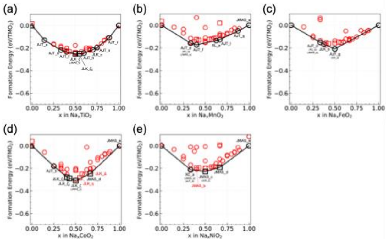
Figure S3. Convex-hull diagrams of the single-TM systems \text{Na}_x\text{TMO}_2 (TM = Ti, Mn, Fe, Co, Ni). Formation energy per \text{TMO}_2 formula unit, referenced to the tie-line between the most stable fully sodiated and fully desodiated endpoints (endpoints at \Delta E = 0 ). Marker shape denotes the host stacking (circle O3, square P3, triangle O1); black-outlined markers are hull ground states, red-outlined markers lie above the hull.
