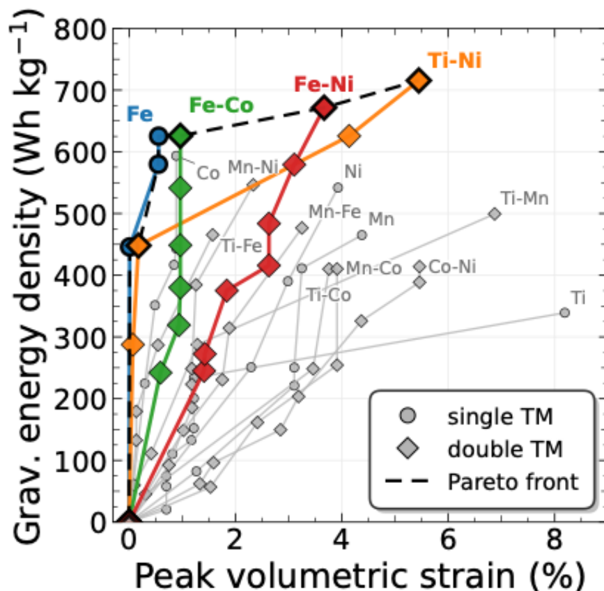
Figure 6. Estimated gravimetric energy density versus peak volumetric strain for all fifteen systems in Figure 2 (circles: single TM; diamonds: double, mixed TM). We integrate the energy density over the computed voltage profile from x = 1 to the lowest-Na stable composition with x > 0 , and we take the peak strain along the same desodiation path. The fully desodiated end member ( x = 0 ) is excluded because of its large volume contraction. Colored markers with black outlines, connected by the dashed line, form the Pareto front.
