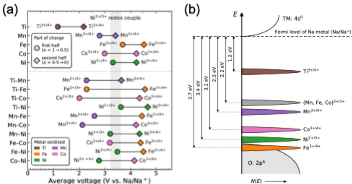
Figure 4. (a) Average voltage of each redox couple over the first (circles) and second (diamonds) halves of charge, calculated from the stable compositions in Figure 2 . Colors identify the oxidized transition metal, labels give the active redox couple, and the gray band marks the voltage range of the Ni 2+/3+ couple. (b) Schematic energy diagram of the redox couples relative to the Fermi level of Na metal (Na/Na + ). Only the depths of the couples are to scale, set by their average first-half voltages from panel (a). N(E) density of states.
