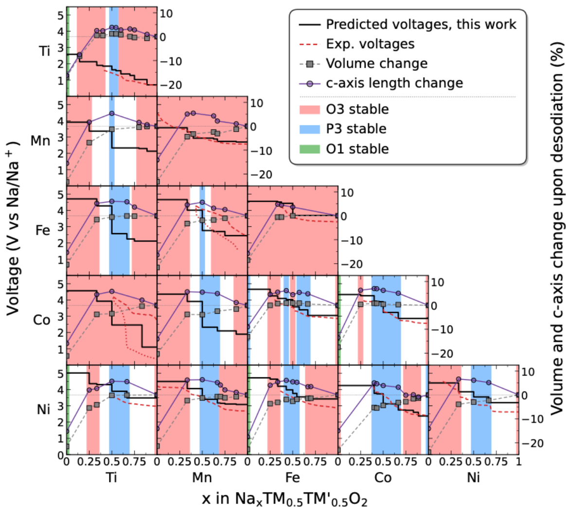
Figure 2. Predicted voltage profiles and volume and c-axis length changes of single- and mixed-transition-metal \text{Na}_x\text{TMO}_2 cathodes , with single-metal \text{Na}_x\text{TMO}_2 arranged along the diagonal, and equimolar \text{Na}_x\text{TM}_{0.5}\text{TM}'_{0.5}\text{O}_2 ; TM = Ti, Mn, Fe, Co, Ni as off-diagonal elements. Black lines display 0 K DFT-predicted voltage (left axis); gray dashed lines show the cell volume per \text{Na}_x\text{TMO}_2 formula unit (right axis); purple lines with circles show the c-axis length per \text{TMO}_2 layer, i.e. , the stacking period divided by the number of \text{TMO}_2 layers in the cell (right axis); red dashed lines illustrate the experimental galvanostatic profiles where available 13,27,29,41,42,44–48 ; where two experimental curves are shown (dashed: charge, dotted: discharge), both are plotted because of the large hysteresis reported in the experiment. Background shading illustrates thermodynamically stable stacking (O1 green, O3 red, P3 blue).
