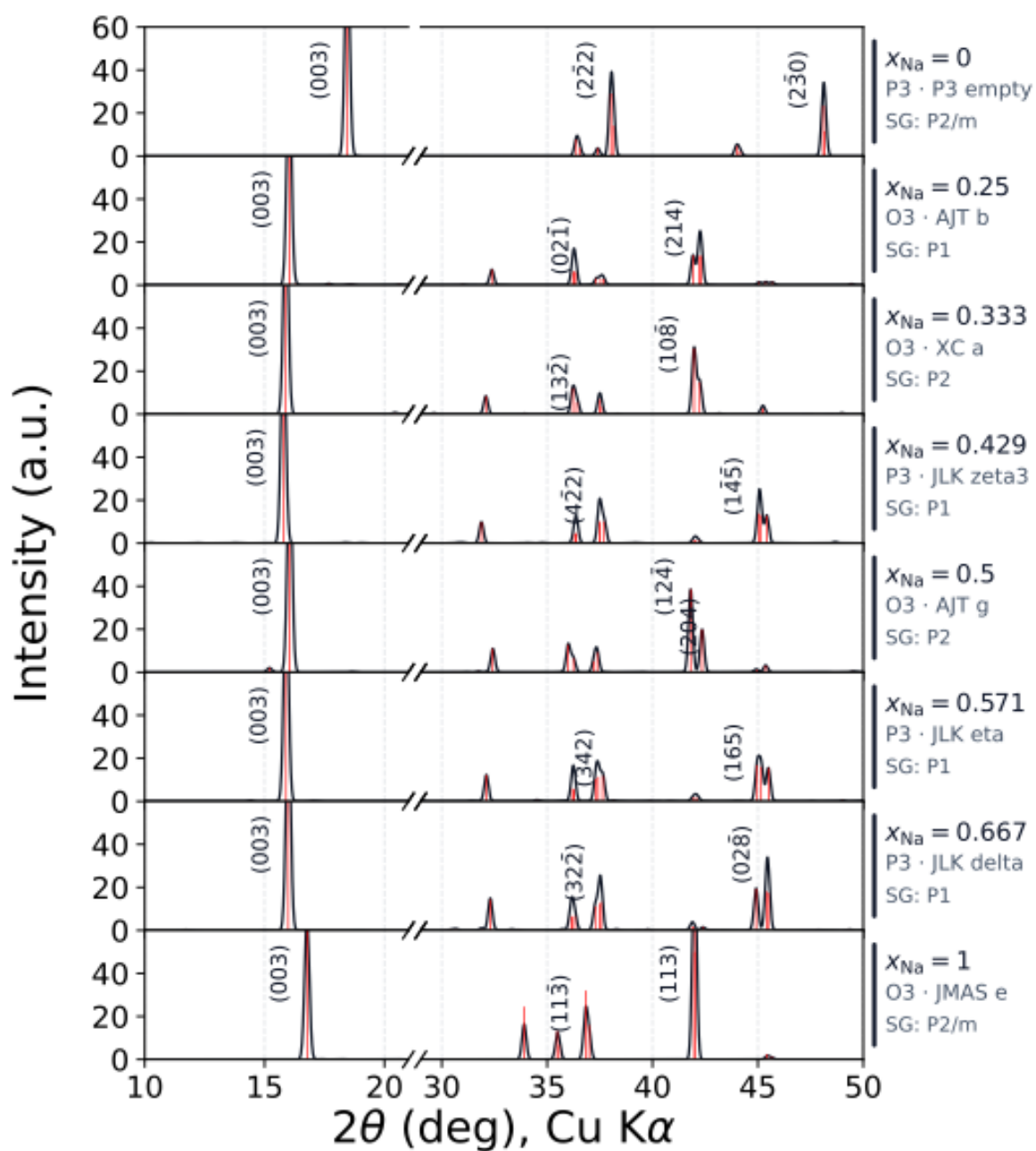
Figure S7 (continued). (h) \text{Na}_x\text{Fe}_{0.5}\text{Co}_{0.5}\text{O}_2 .
