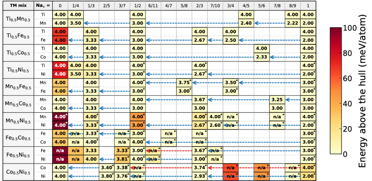
Figure 3. Predicted average TM oxidation states and thermodynamic stability of mixed \text{Na}_x(\text{TM})_{0.5}(\text{TM}')_{0.5}\text{O}_2 systems vs. Na content x (two rows per pair: TM top, TM' bottom). Colors show the energy above the convex hull (meV/atom) of each composition relative to the phases in the Materials Project database. Numbers give the average oxidation state of each transition metal, inferred from the DFT on-site magnetic moments; "n/a" marks compositions where the assigned oxidation states violate charge neutrality. Arrows mark redox-active elements during desodiation: blue for oxidation, red for reduction. Asterisks mark stable compositions within the Na range reached by electrochemical (de)sodiation in experiments 41,42,45–47,53 .
