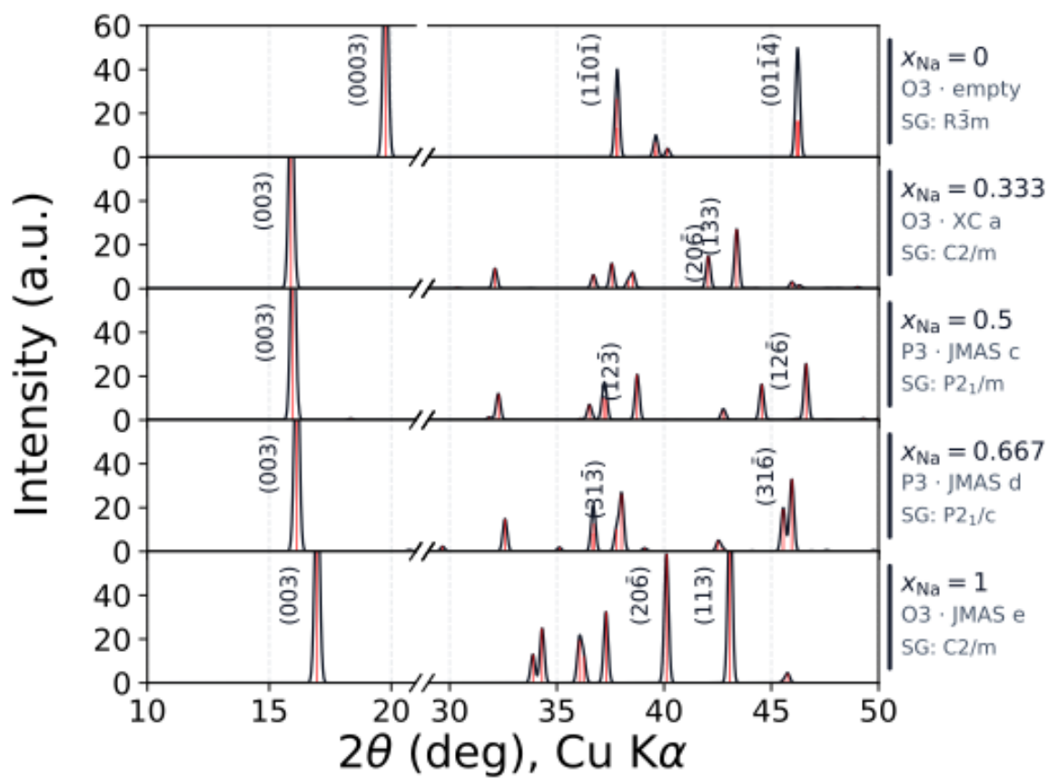
Figure S6 (continued). (e) \text{Na}_x\text{NiO}_2 .
