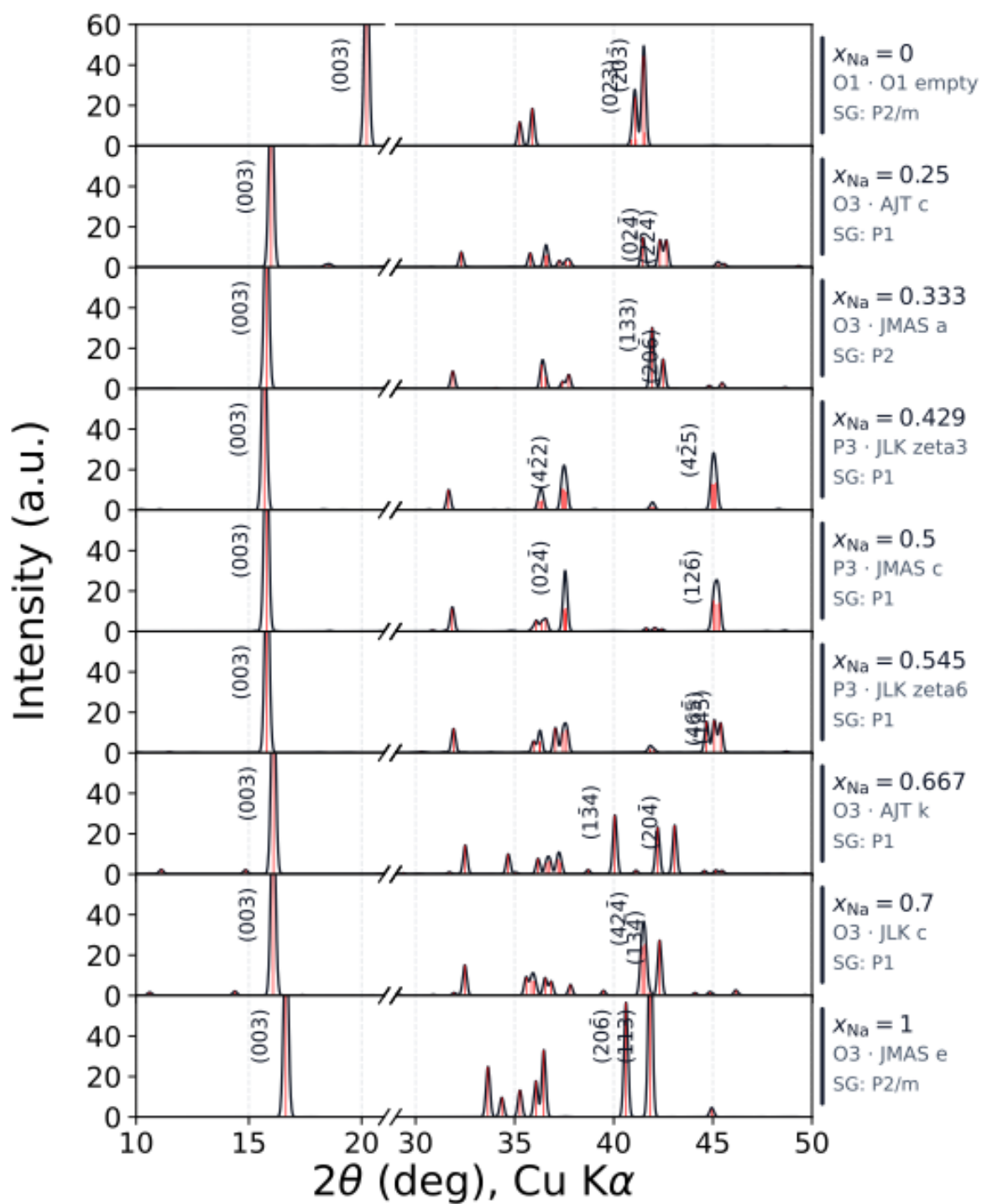
Figure S7 (continued). (i) \text{Na}_x\text{Fe}_{0.5}\text{Ni}_{0.5}\text{O}_2 .
