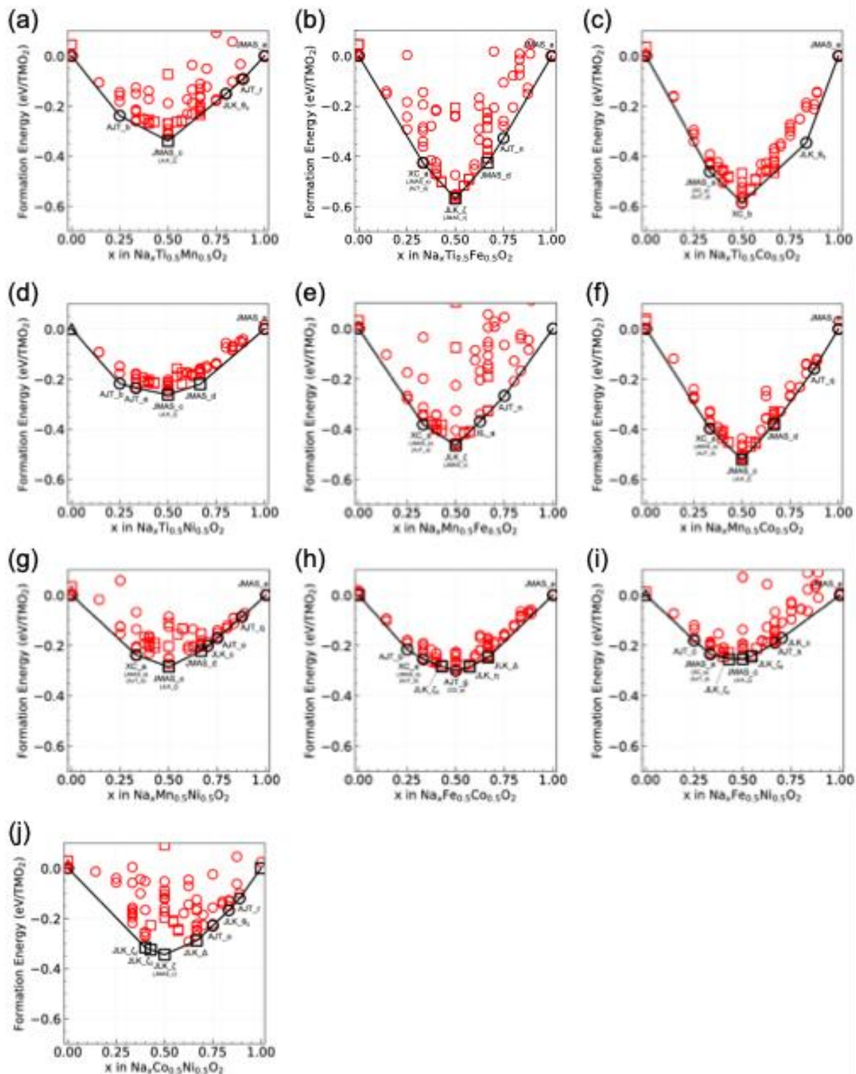
Figure S4. Convex-hull diagrams of the ten mixed systems \text{Na}_x\text{TM}_{0.5}\text{TM}'_{0.5}\text{O}_2 , plotted as in Figure S3.
