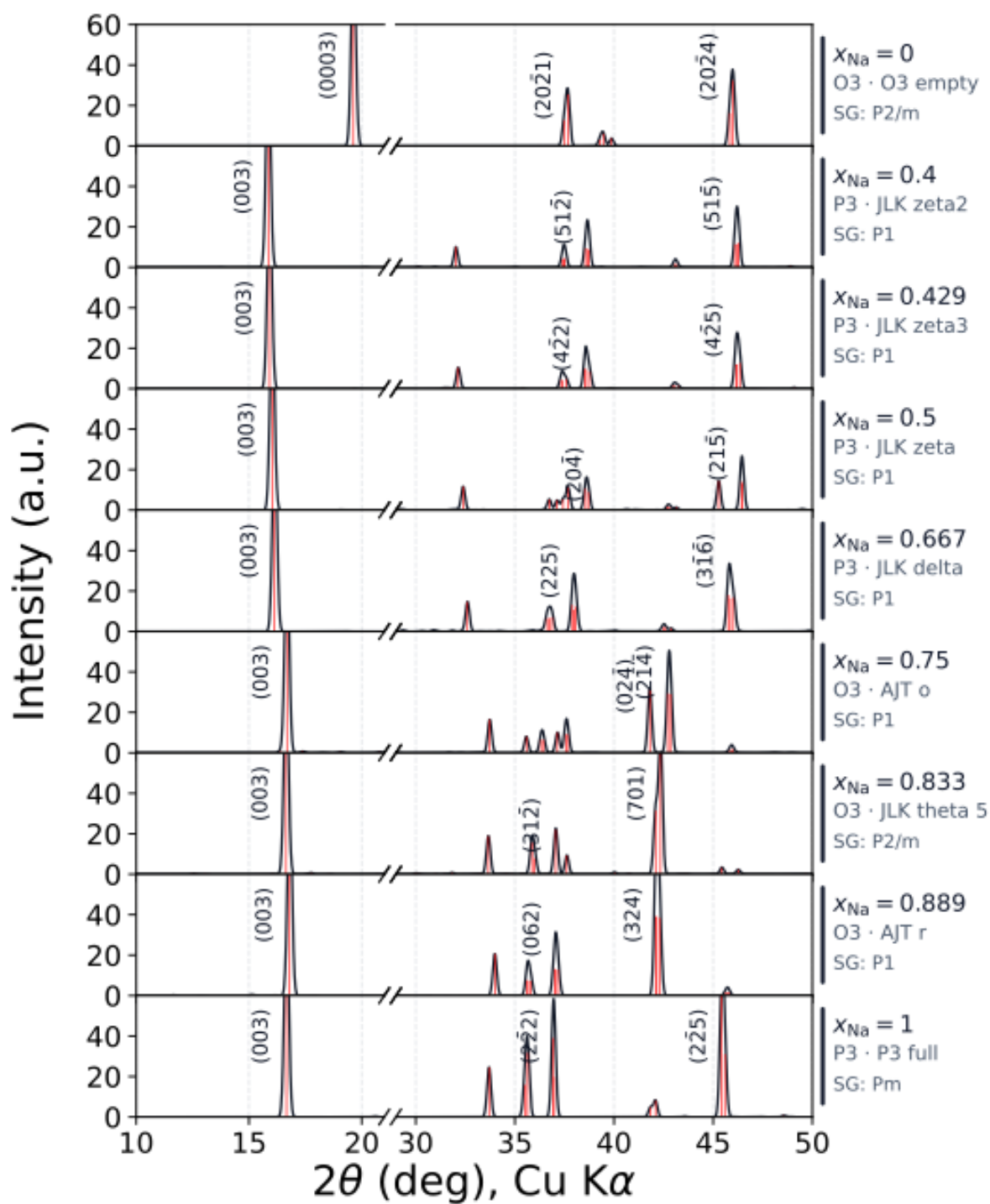
Figure S7 (continued). (j) \text{Na}_x\text{Co}_{0.5}\text{Ni}_{0.5}\text{O}_2 .
