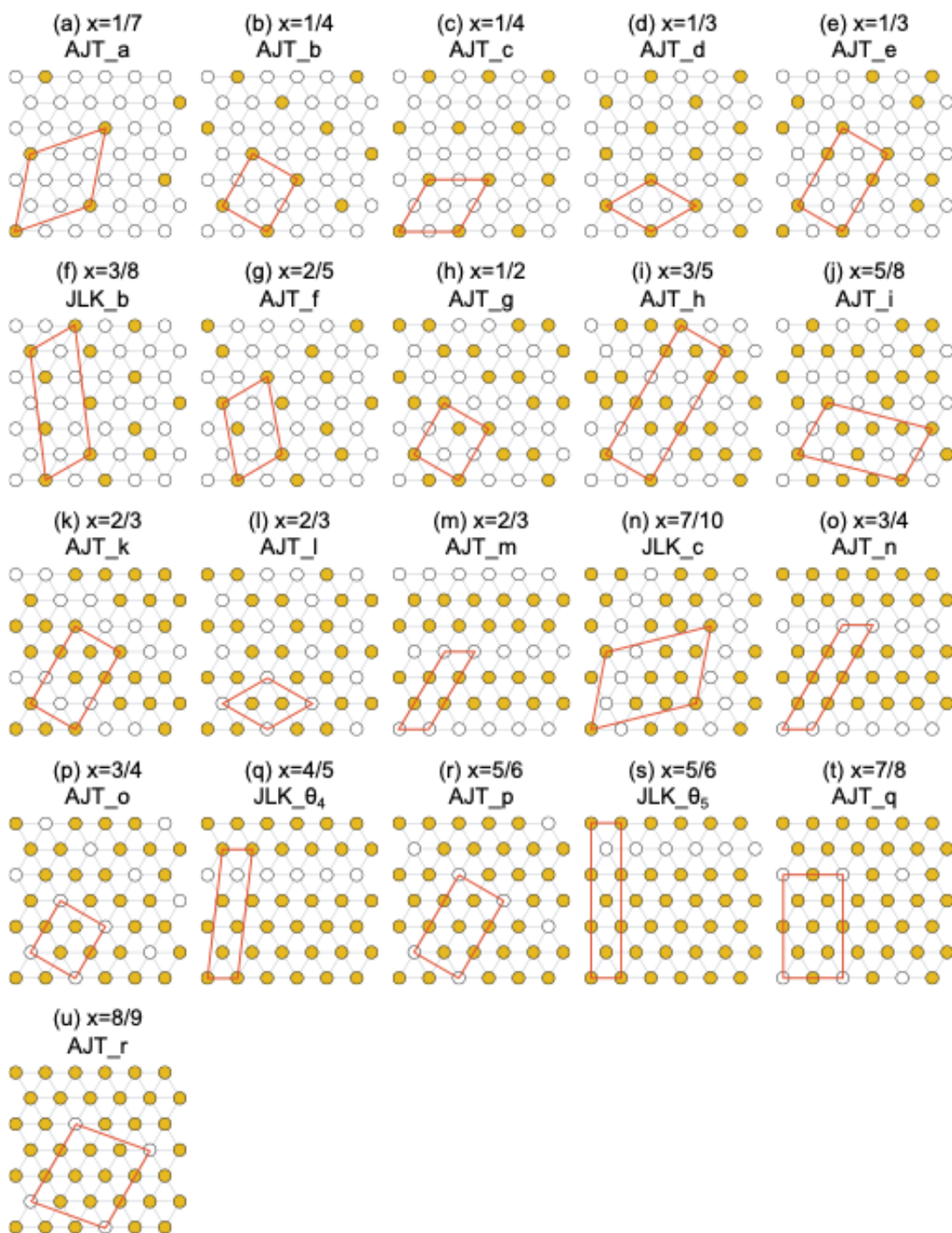
Figure S1. Na-vacancy ordering diagrams of the O3-host orderings used in the DFT calculations. Labels of each ordering encode provenance: the initials of the authors of the source study, followed by the ordering label used in that work, or by an alphabetic index where the source did not label its orderings (AJT: Toumar et al. 2015 1 ; JLK: Kaufman & Van der Ven 2019 and 2022 2,3 ; JMAS: Steele et al. 2025 and 2026 4,5 ; XL: Li et al. 2014 6 ; XC: Chen et al. 2018 7 ; CD: Didier et al. 2012. 8 Orderings identical to a listed entry up to a monoclinic lattice distortion are omitted: XC_a and JMAS_a are variants of AJT_d, JMAS_b of AJT_f, and CD_a of AJT_g. XC_b and XL_a are omitted because small off-site Na displacements take their Na-vacancy orderings off the ideal triangular lattice.
