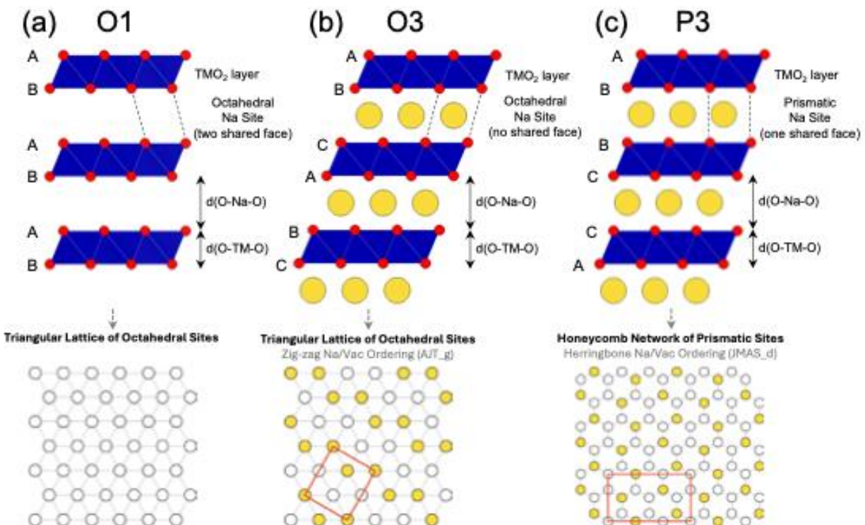
Figure 1. Three-layer stacking models of \text{Na}_x\text{TMO}_2 in the Delmas notation 22 : (a) O1, (b) O3, and (c) P3, with the oxygen stacking sequence labeled on each panel. Blue: \text{TMO}_6 octahedra forming \text{TMO}_2 slabs; red: O; yellow: Na; arrows: interslab distance d(\text{O-Na-O}) and d(\text{O-TM-O}) . Bottom row: in-plane Na site networks. The orderings in (b) and (c) are one example each of the many possible Na/Vac orderings (filled/open circles: occupied/vacant sites; red outline: unit cell; all orderings in Figures S1 and S2 ). The O1 phase is shown as an empty network, as it appears only near full desodiation.
