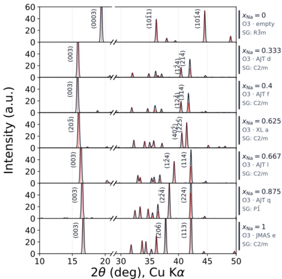
Figure S6 (continued). (b) \text{Na}_x\text{MnO}_2 .
