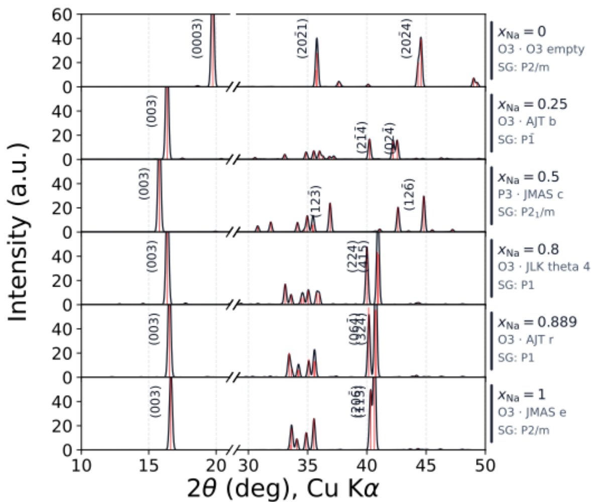
Figure S7. Simulated XRD patterns (Cu K \alpha ) of every hull-stable structure of the ten mixed systems of Figure S4, presented as in Figure S6 (one TM pair per page). (a) \text{Na}_x\text{Ti}_{0.5}\text{Mn}_{0.5}\text{O}_2 .
