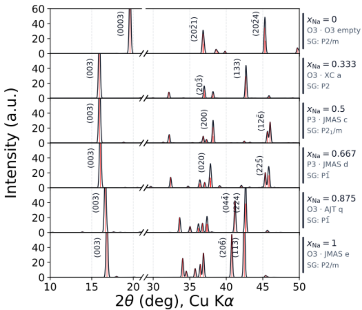
Figure S7 (continued). (f) \text{Na}_x\text{Mn}_{0.5}\text{Co}_{0.5}\text{O}_2 .
