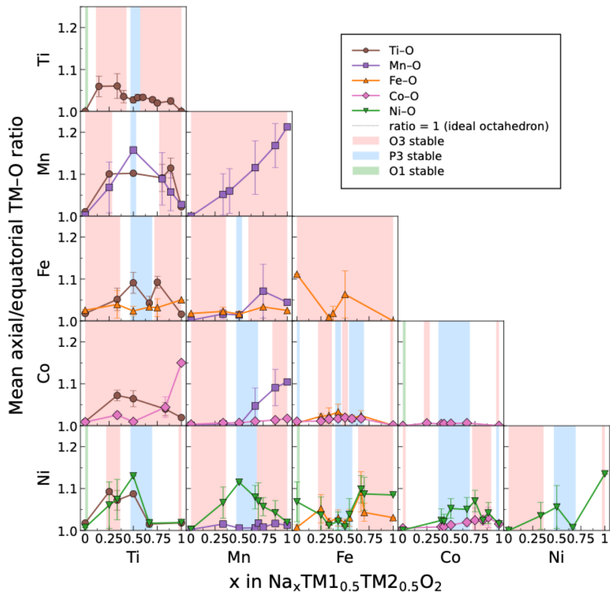
Figure S5. Jahn-Teller distortion of the \text{TMO}_6 octahedra versus Na content, quantified as the mean axial-to-equatorial TM-O bond-length ratio (two longest bonds = axial, four shortest = equatorial; 1.0 = ideal octahedron, >1 = JT elongation), averaged over all octahedra of each element. Error bars: standard deviation across the symmetry-distinct octahedra of that element. Markers color/shape-coded by element; shading: stable stacking (O3 red, P3 blue, O1 green).
